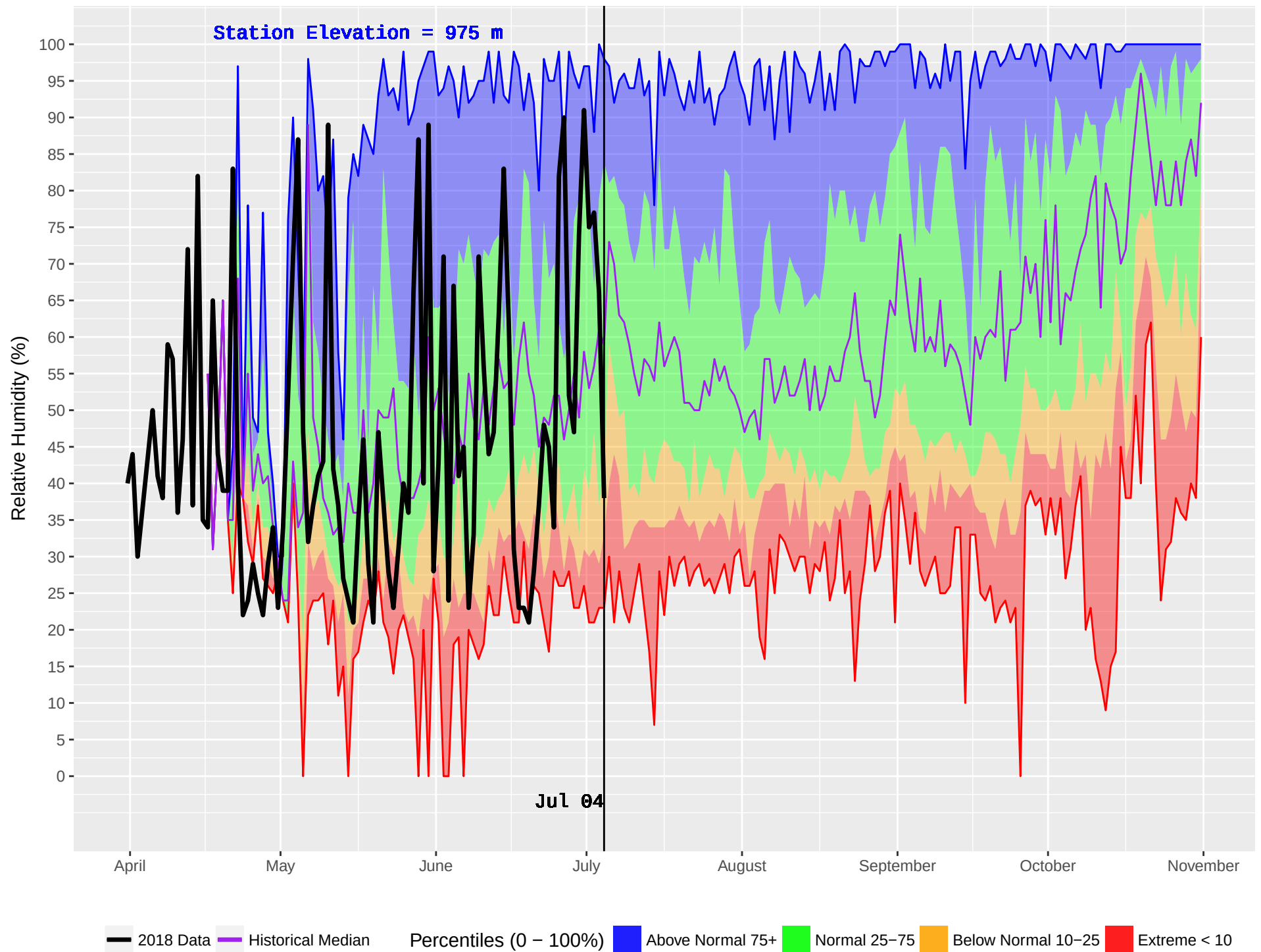
MCGREGOR 2 (192) : Historical (1986–2016) and Current (2018) Noon Relative Humidity
