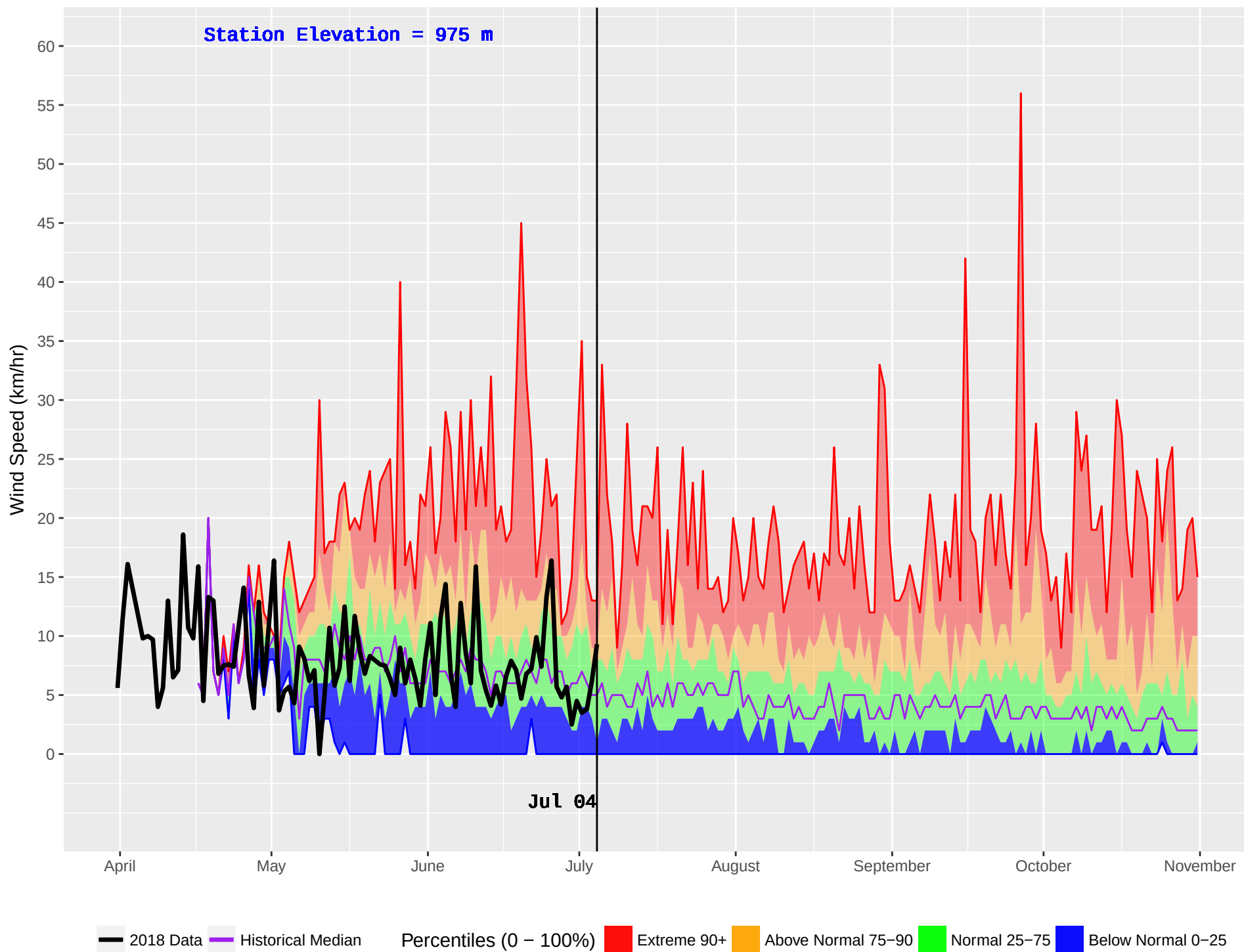
MCGREGOR 2 (192) : Historical (1986–2016) and Current (2018) Noon Wind Speed
