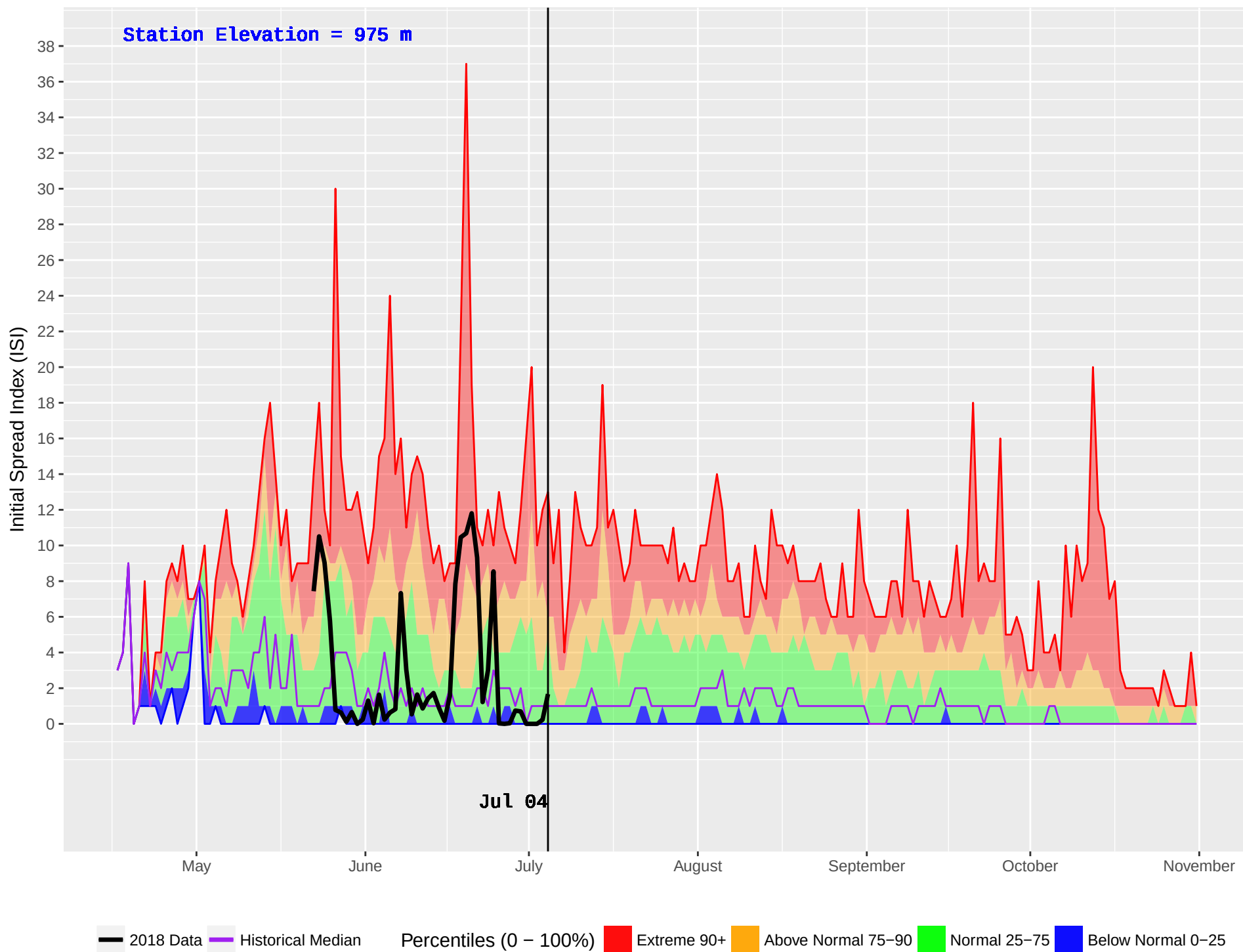
MCGREGOR 2 (192) : Historical (1986–2016) and Current (2018) Noon Initial Spread Index (ISI)
