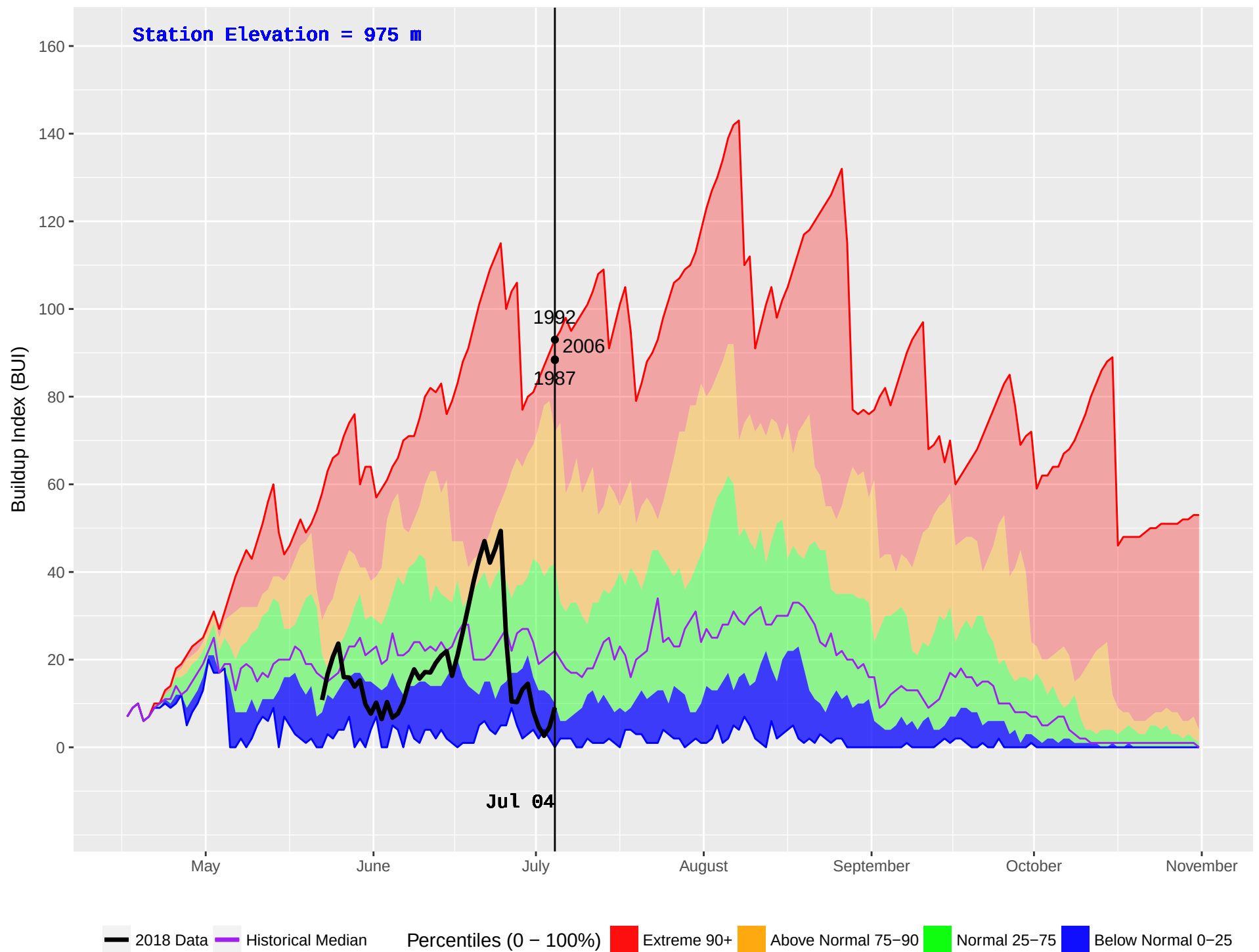
MCGREGOR 2 (192) : Historical (1986–2016) and Current (2018) Noon Buildup Index (BUI)
