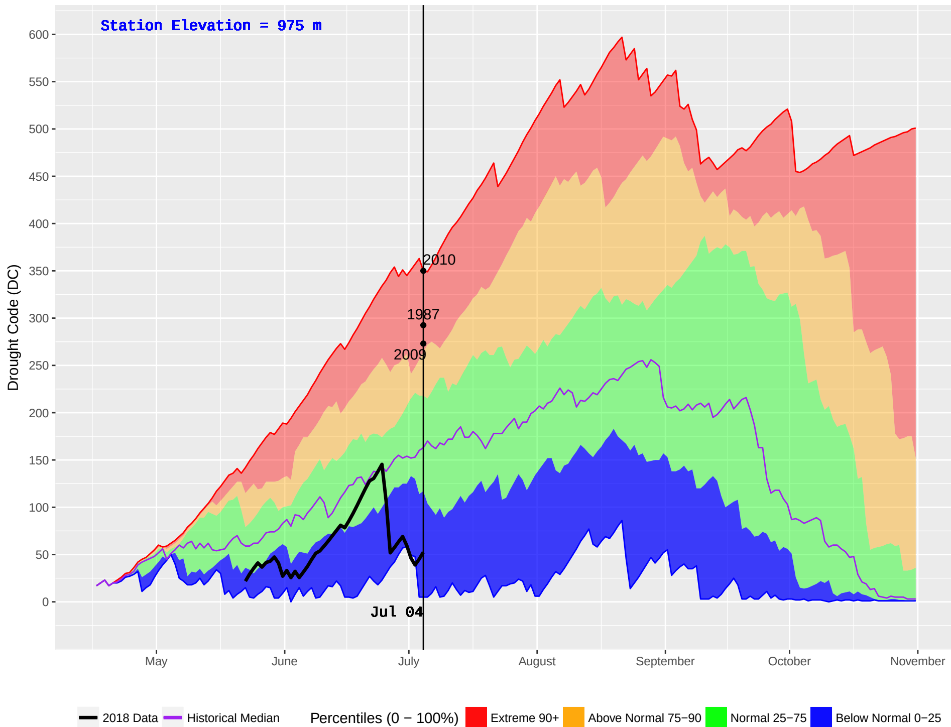
MCGREGOR 2 (192) : Historical (1986–2016) and Current (2018) Noon Drought Code (DC)
