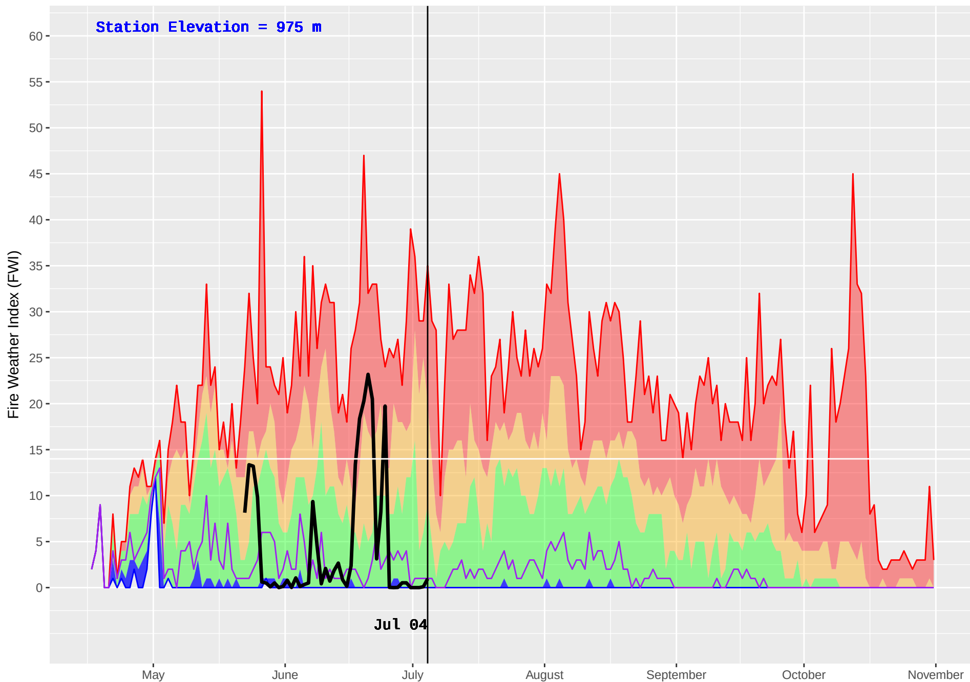
MCGREGOR 2 (192) : Historical (1986–2016) and Current (2018) Noon Fire Weather Index (FWI)
